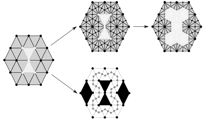
Fig. 4: Two equivalent computations of a separation. The first approach consists of a subdivision followed by a “thickening”; the dashed line is then the separation we are seeking. The second approach consists of computing the barycenters of the simplices whose at least one vertex is white and at least one vertex is black and joining these barycenters by edges.
