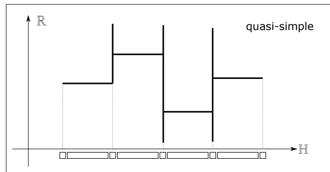
Fig. 24: An example of quasi-simple map on the 1D Khalimsky grid \mathbb{H} : we can observe that this map U is USC, that for any x in the domain of U , the set U(x) is connected and closed, and that U(x) is “flat” on the maximal faces.
