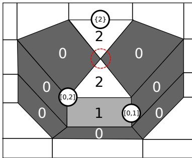
Fig. 12: The initial image U : X \rightarrow \mathbb{I}_{\mathbb{R}} , containing a pinch encircled in red: at this vertex, the boundary of [U > 1] crosses itself. Circles indicate the values of the span-valued map U on some of the k -faces of X ( k < n ).
