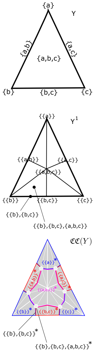
Fig. 29: Computation of a cell-complex: a simplicial complex Y , its first subdivision Y^1 , and the computation of the dual of the first subdivision, that is, \mathcal{CC}(Y) ; the thin lines in the last figure correspond to Y^2 .
