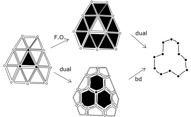
Fig. 30: The dual of the frontier order is equal to the boundary of the dual. We start from a set of points \Lambda_X (the 3 points in black in the left subfigure), a set \Lambda_C (the 12 black and white points in the same subfigure), and a simplicial complex C (this same figure in totality). Then, we obtain the frontier order of \Lambda_X in \Lambda_C relative to C in the top-middle subfigure in black. Then, we compute its dual and we obtain the simple closed curve (in the right subfigure). Restarting from the set X (in black in the left subfigure), we compute its dual and we obtain the black poset made of 3 hexagons, 3 edges, and one vertex (see the middle-bottom figure). Finally, we compute its boundary and we obtain the same simple closed curve as before.
