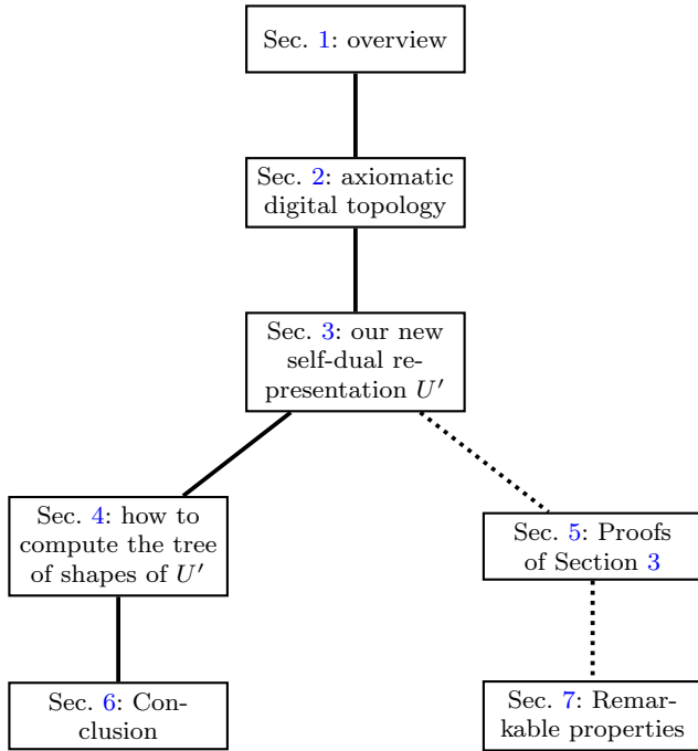
Fig. 5: The scheme of the whole paper. Note that Section 5 and Section 7 are optional for the intuitive understanding of the paper.
