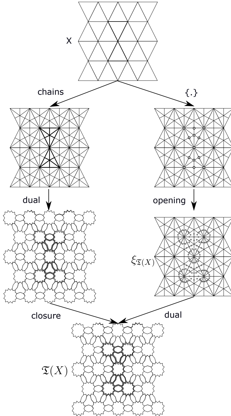
Fig. 32: Starting from the simplicial complex X resulting from the closure of two triangles sharing a vertex in a 2-surface |Y| , we compute on the left side the closure in \mathcal{CC}(Y) of the complex \mathcal{CC}(X|Y) and on the right side the dual of the set \xi_{\mathfrak{T}(X)} . Both lead to \mathfrak{T}(X) .
