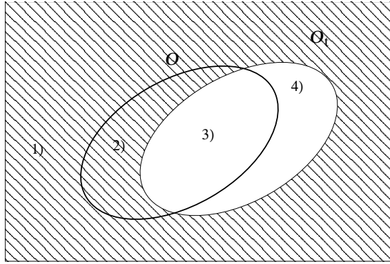
Figure 4: The case of translations.
