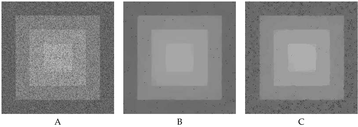
Figure 7: A: original noisy image (Rayleigh speckle noise)- B: result with TV - C: result with adapted levelable function.
