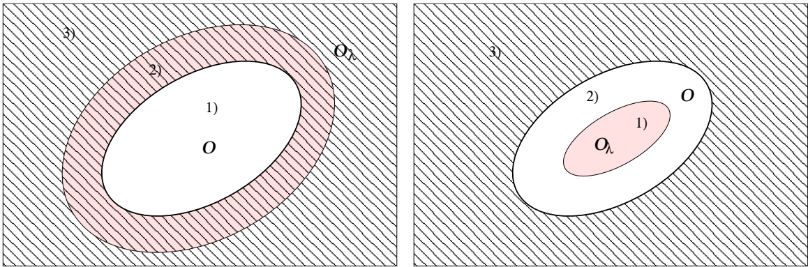
Figure 1: Homothecies. Left : case I) - Right : case II) .
