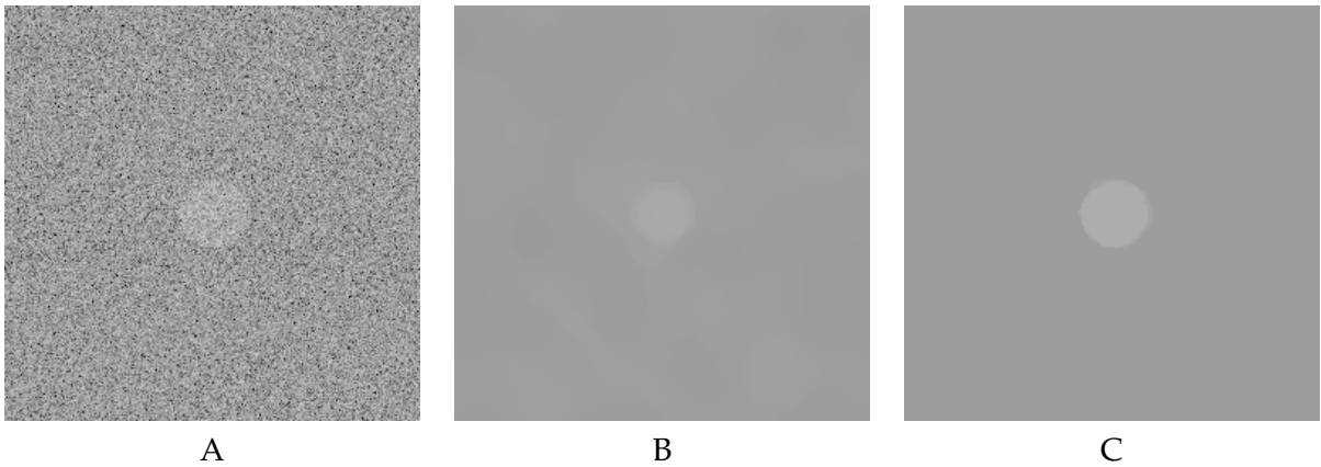
Figure 5: A: original noisy image (Gaussian noise) - B: result with TV - C: result with adapted levelable function.
