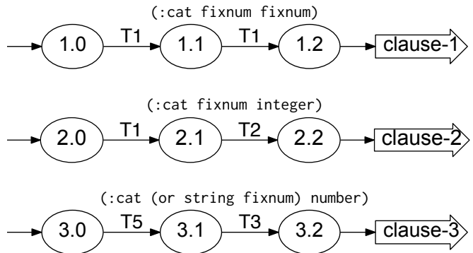
Figure 6: The rte representing the destructuring-bind and type declarations from Figure 5.
