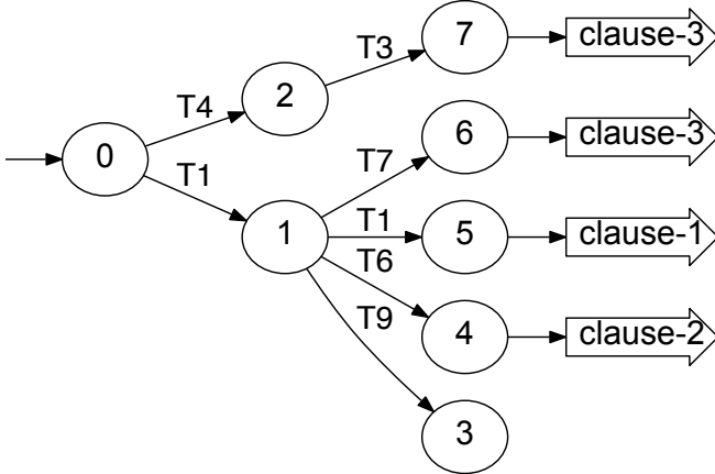
Figure 10: Transition Computation for dfa 2 × dfa 3
