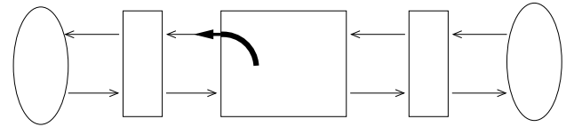
Figure 2: Perception Generation
