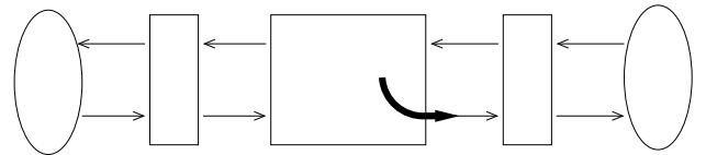
Figure 7: Action Generation
